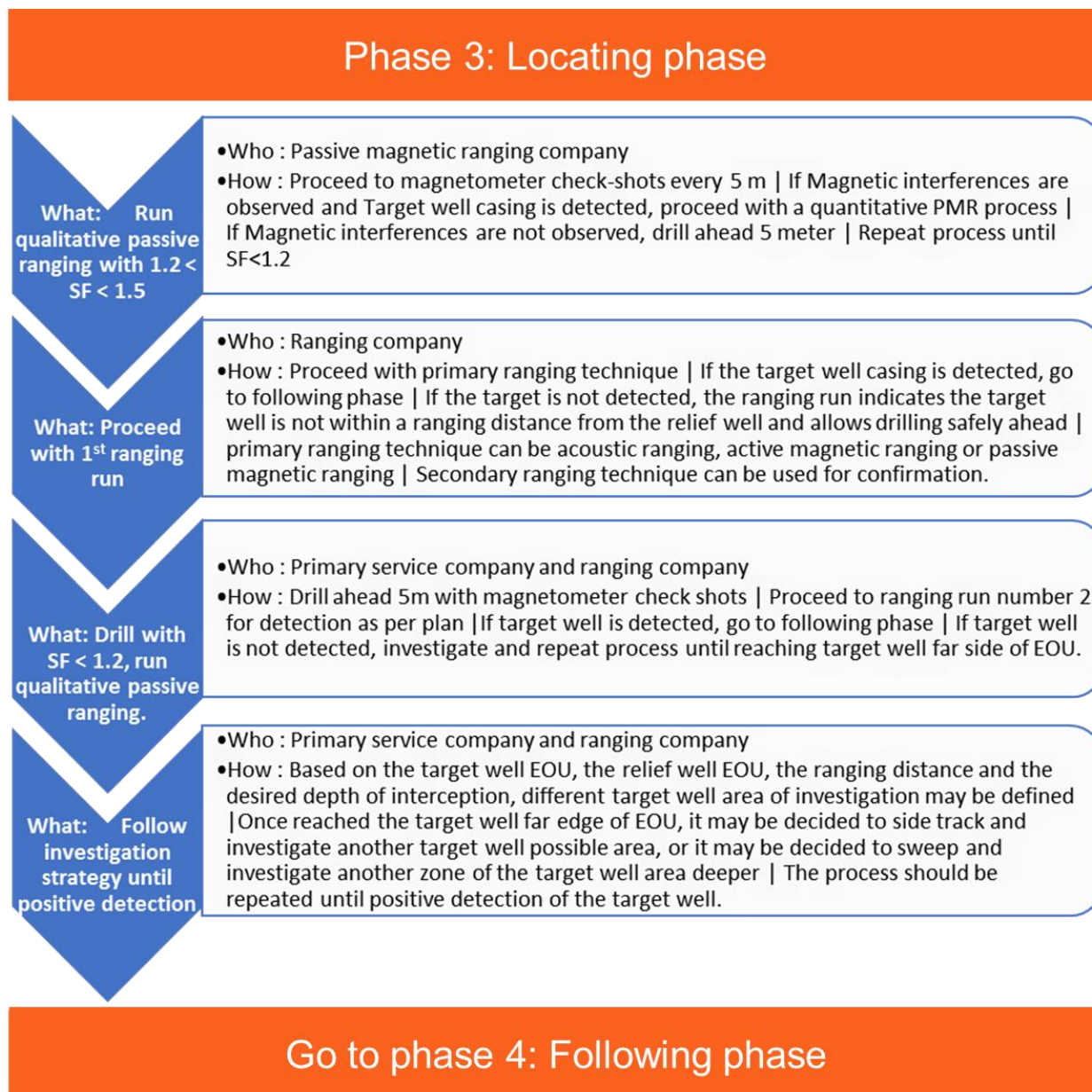
Figure 70—Phase 3: Locating phase key tasks and responsibilities
