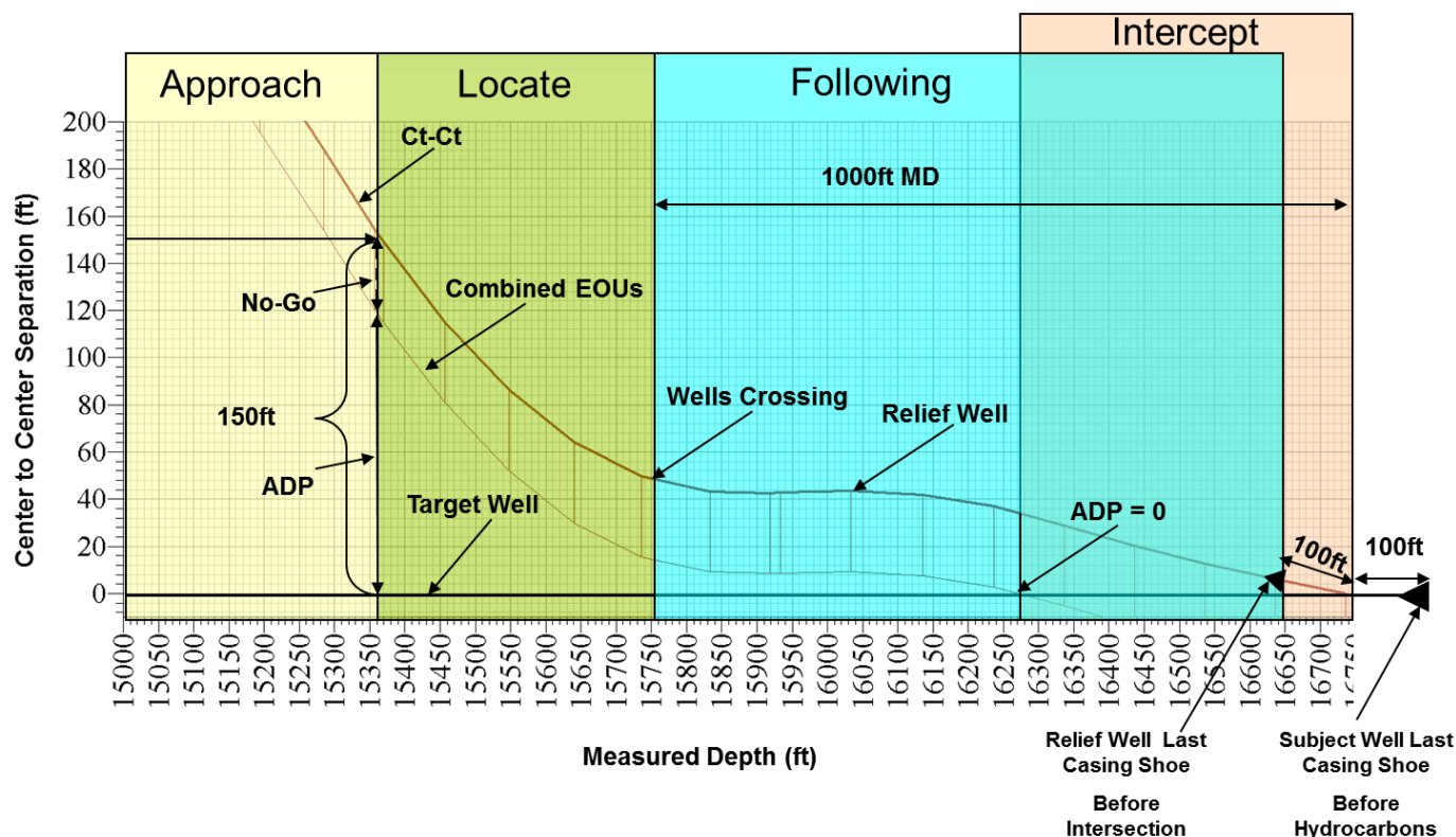
Figure 84—An example of GOM relief well ladder plot, centre-to-centre distance to the target relative to the relief well. Based on MWD + IFR + MS Surveys and BP Major Risk Criteria for the EOU calculation
