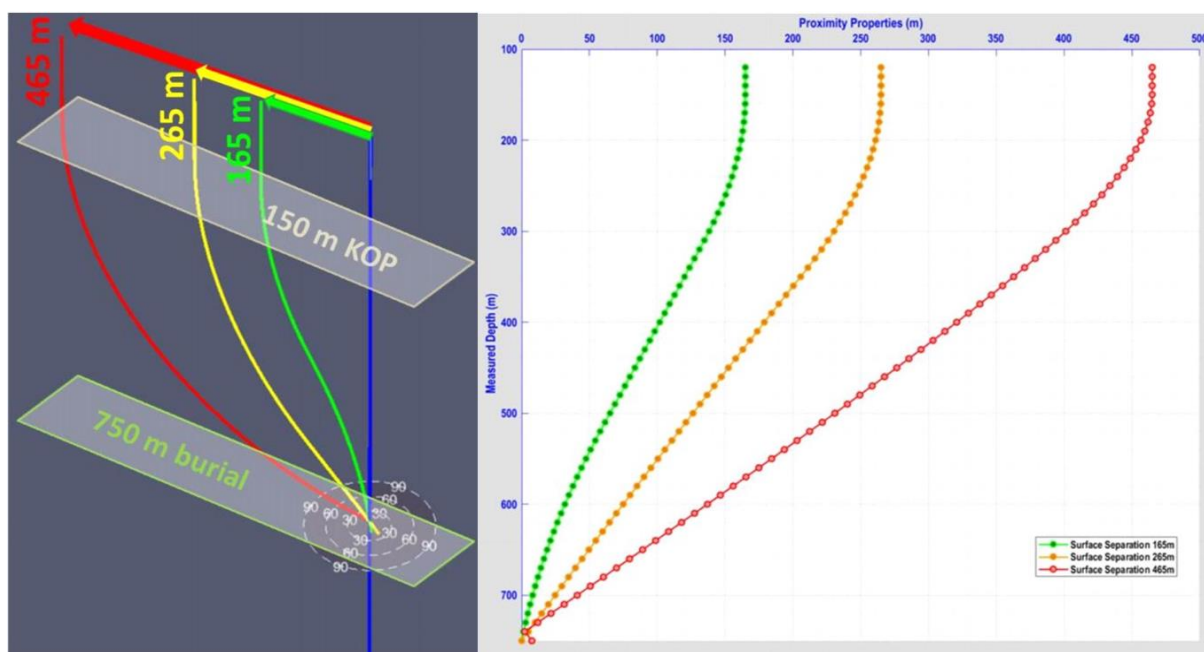
Figure 55 —Surface Location and Drilling Complexity Sensitivity Analysis
