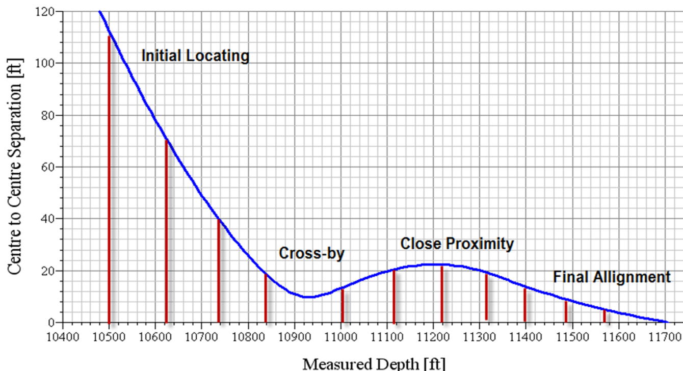
Figure 83 - An example of relief well centre-to-centre distance to the target well plotted by measured depth
