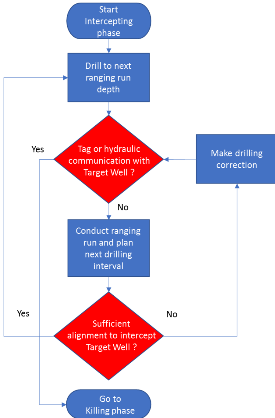
Figure 80—Intersecting phase ranging decision flow chart
