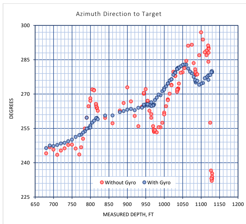
Figure 86—Azimuth direction to target ranging data including the gyro measurements and without gyro measurements at < 2 deg inclination
