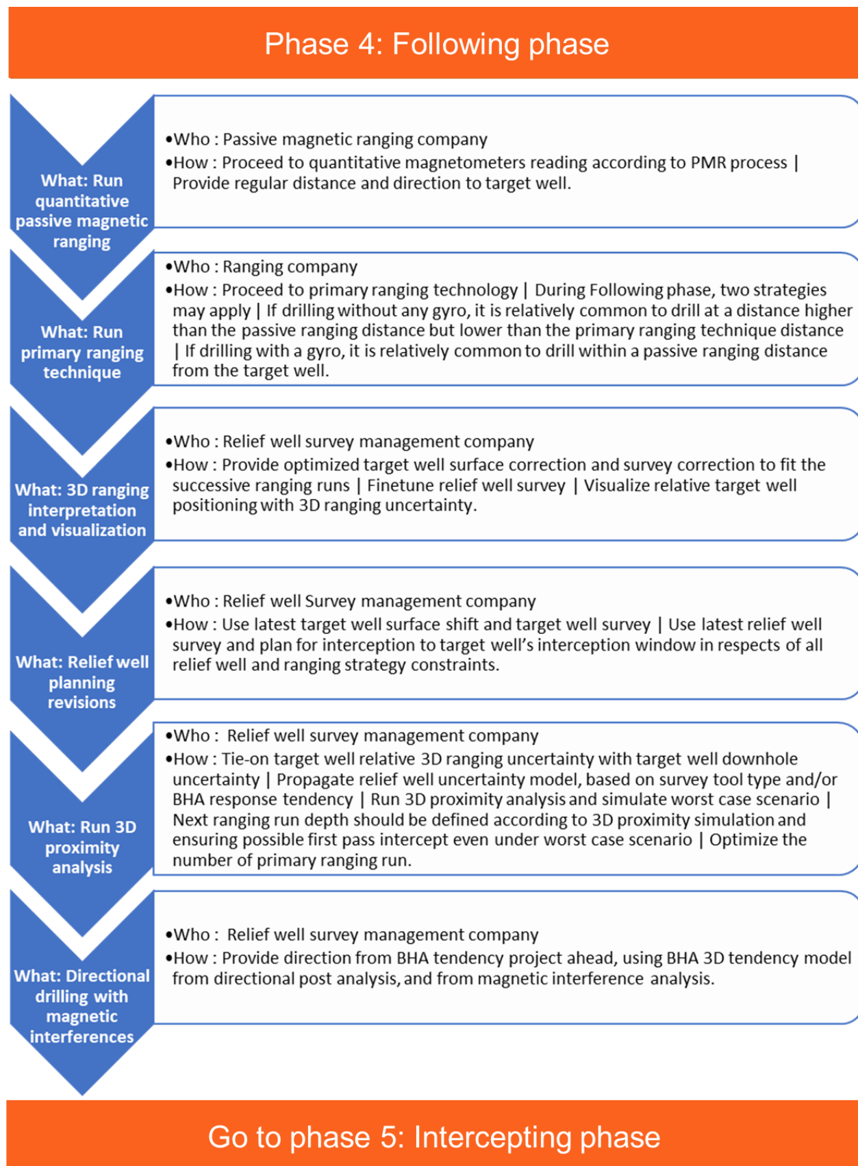
Figure 76—Phase 4: Following phase key tasks and responsibilities
