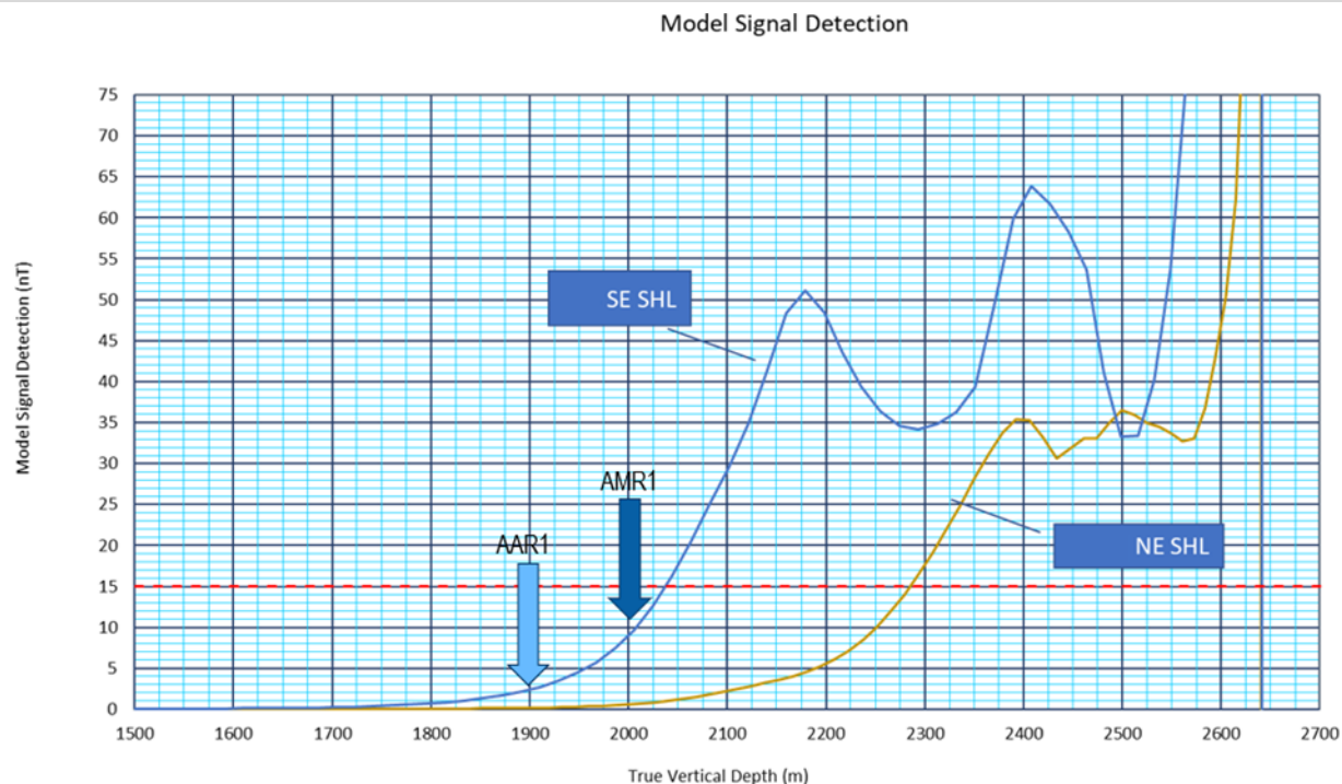
Figure 61—Plot of modelled signal detection in nT versus TVD of the relief well profile. The red dashed line at 15 nT indicates the threshold for detection and it is possible to see that the SE well profile reaches the threshold about 250 meters earlier
