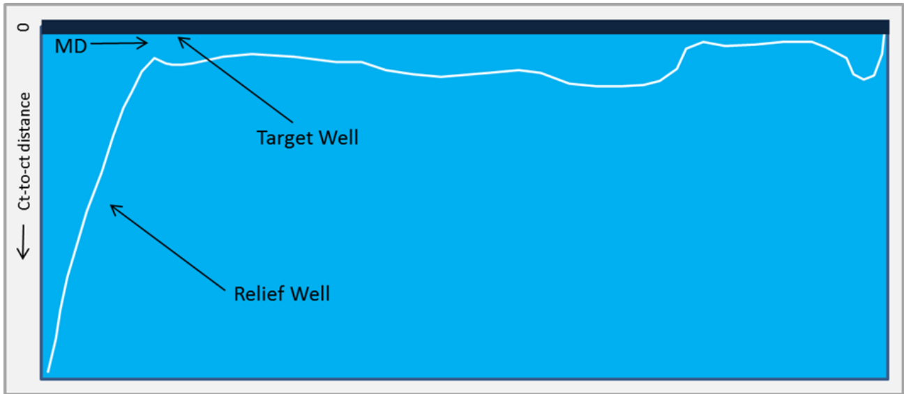
Figure 38—Ct-ct distance between the subject and target wellbore
