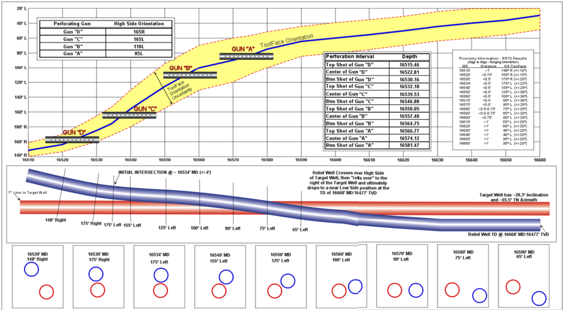
Figure 87—Example perforating method to establish hydraulic communication
