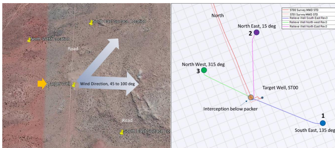
Figure 60 — Possible relief well surface locations. The red line is the plan view of the target well trajectory. Based on kill mud modelling the targeted interception point is at 57 degrees inclination in the curve section.
