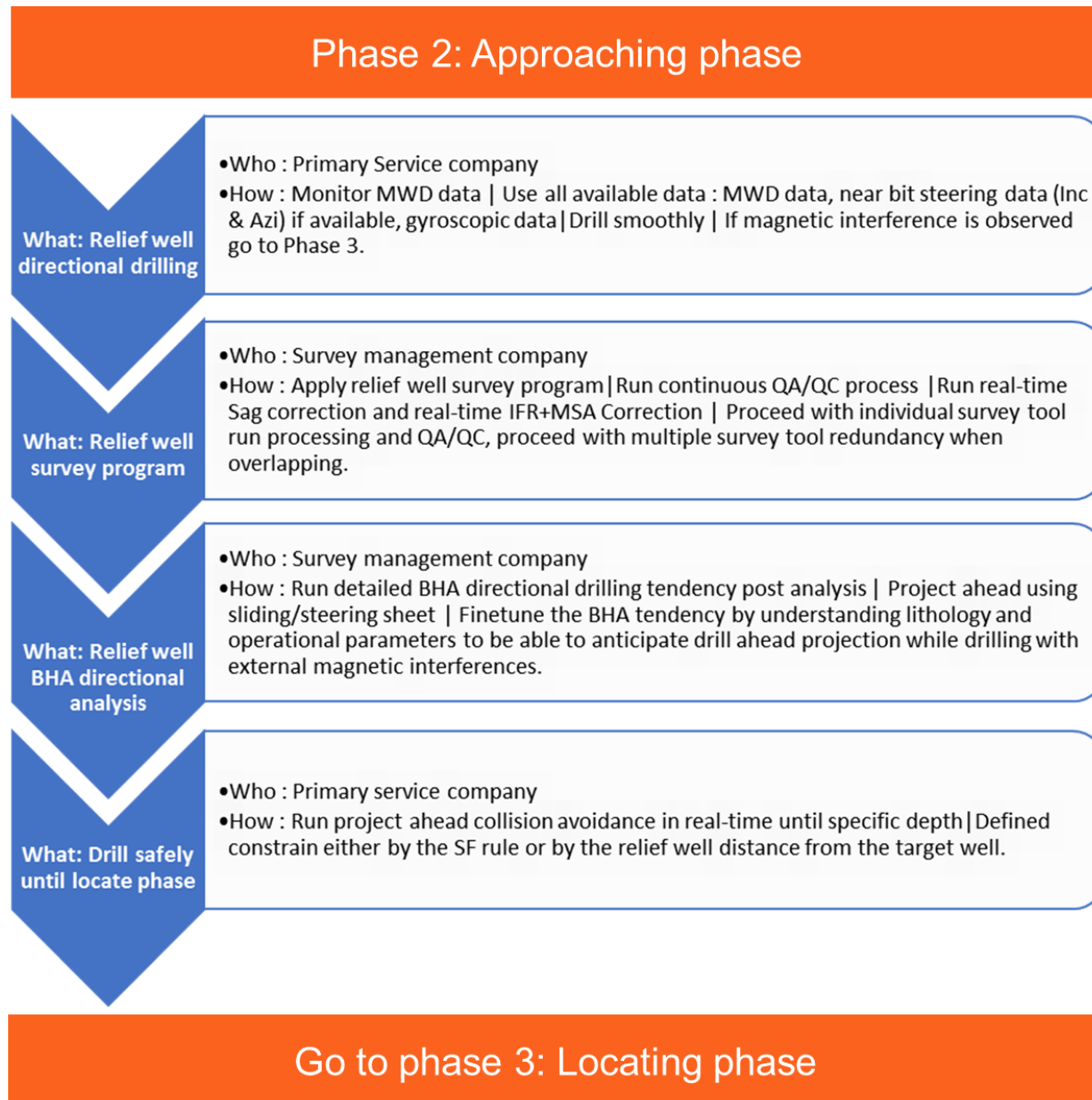
Figure 65—Phase 2: Approaching phase key tasks and responsibilities
