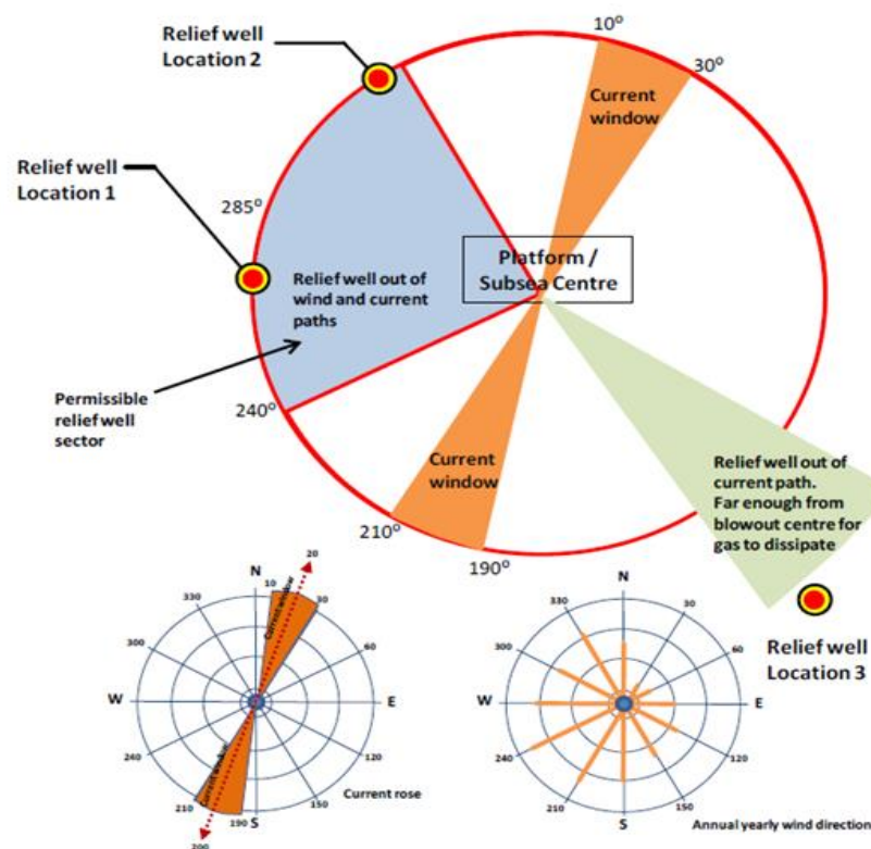
Figure 59—Example of relief well locations based on prevailing wind and current study
