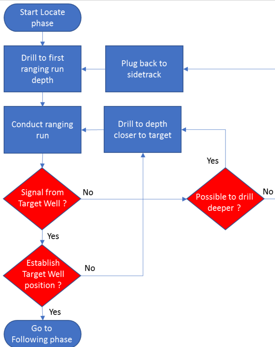
Figure 71—Locating phase ranging decision flow chart
