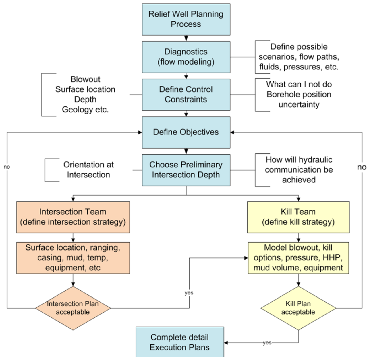
Figure 67—Summarized wellbore interception planning steps
