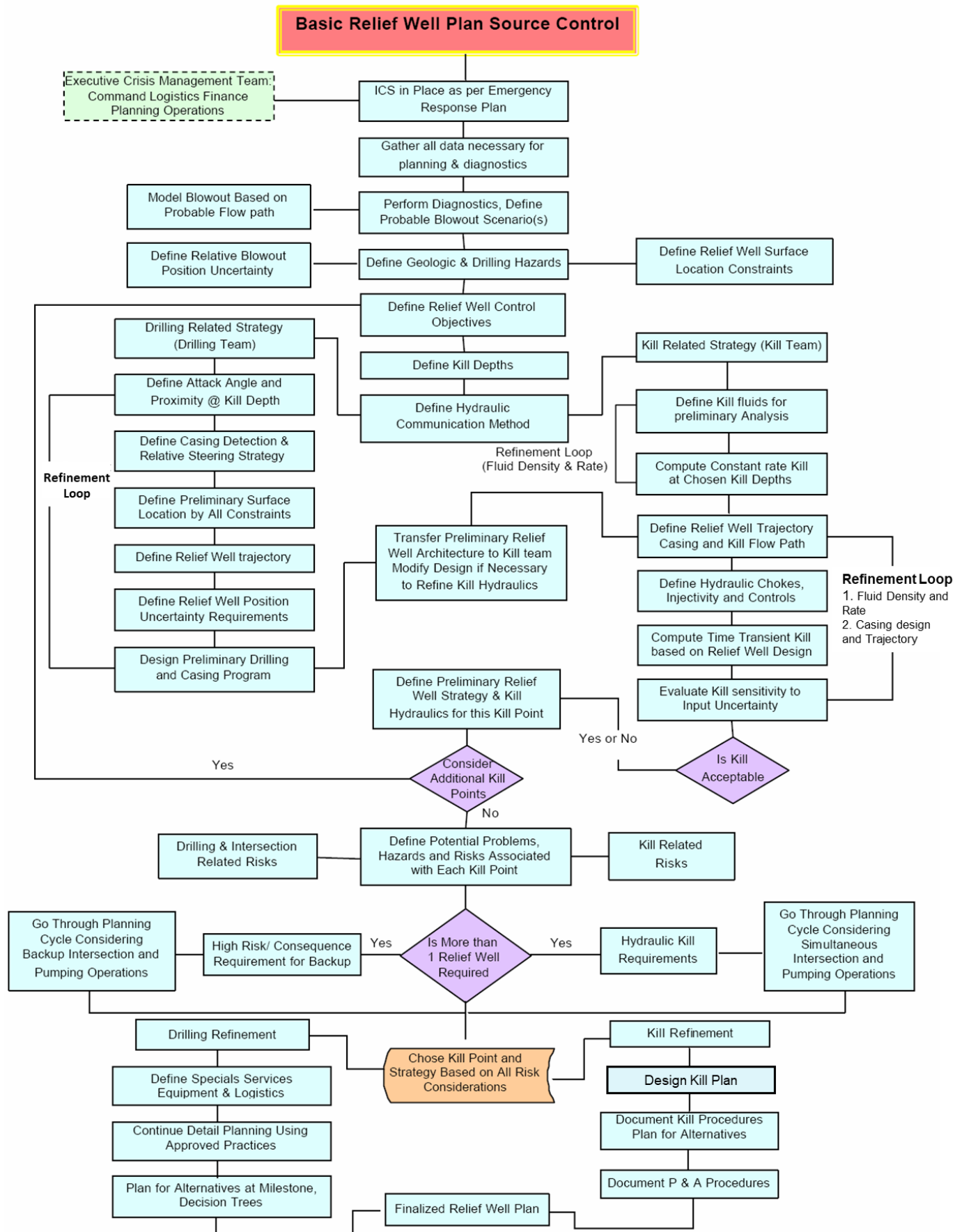
Figure 68—An example of detailed relief well planning process
