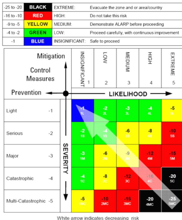
Figure 62—The HARC process identifies and isolates all potential hazards and relates them to the risk of occurrence in addition to the potential impact on the relief well drilling
