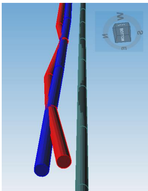
Figure 85—Ranged position of the drilling well (magnetic orientation – red, gyro orientation – blue) relative to the reference offset well (teal).
