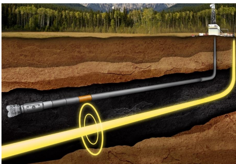
Figure 14—SA-AMR uses well-head access to induce a magnetic field in the target well (shown in yellow above) which is then utilized by a downhole sensor in the drilling BHA
