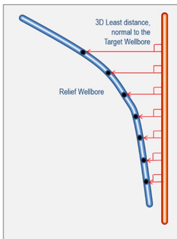
Figure 32—3D least distance illustration
