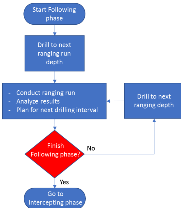
Figure 77—Following phase ranging decision flow chart
