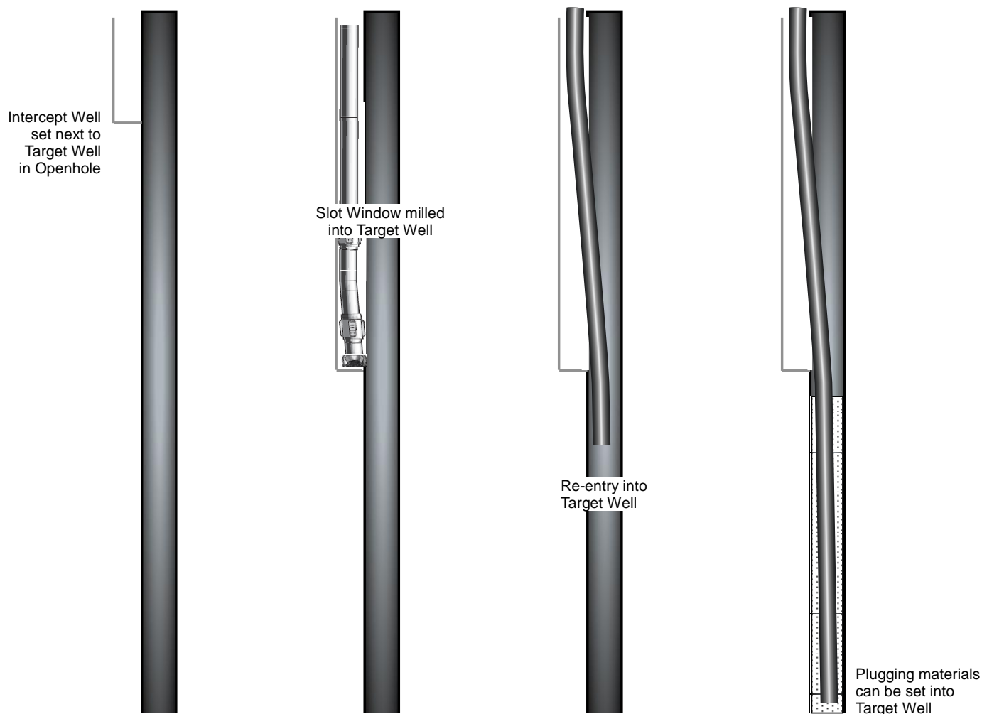
Figure 88—Slot milling method concept
