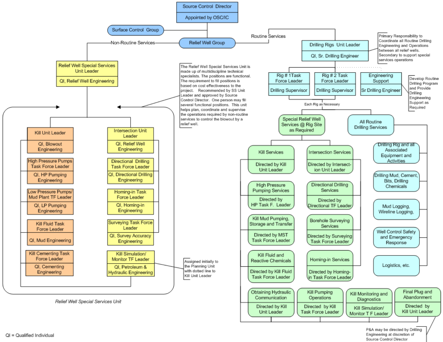
Figure 92—Example of relief well team organization
