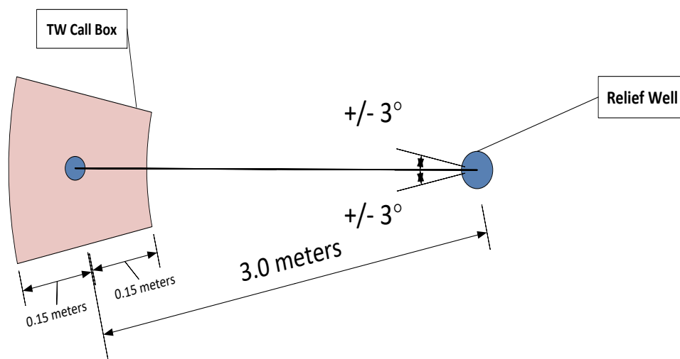
Figure 74—Ranging call with a direction of 270^\circ + 3^\circ and a distance of 3.0 meter + 0.15m
